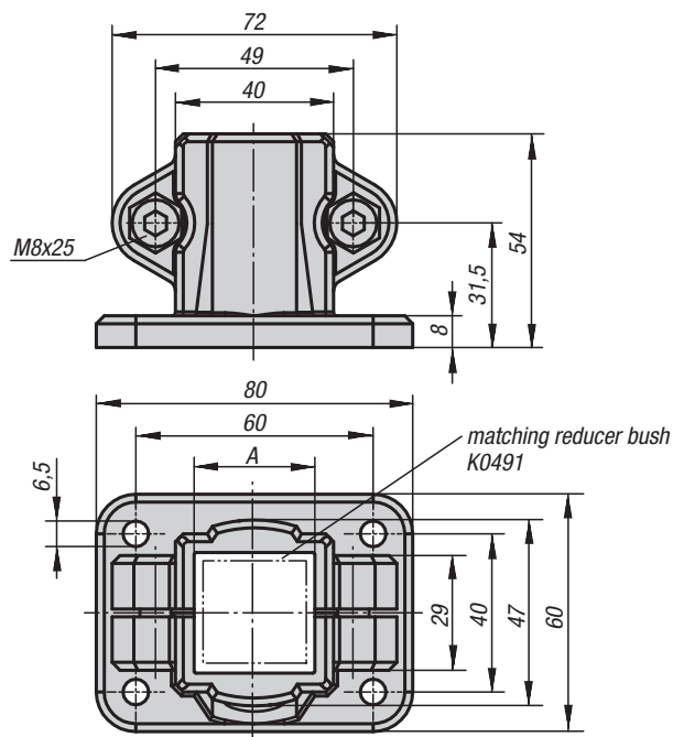
KIPP Base clamp, plastic
