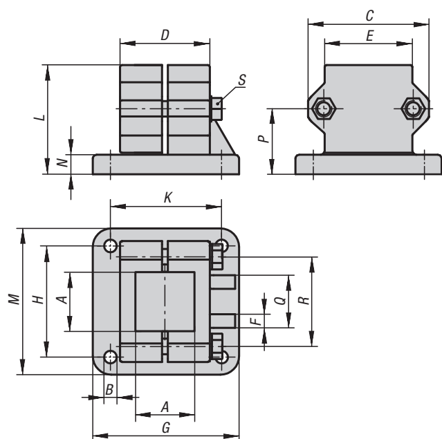
KIPP Base clamps, aluminium
