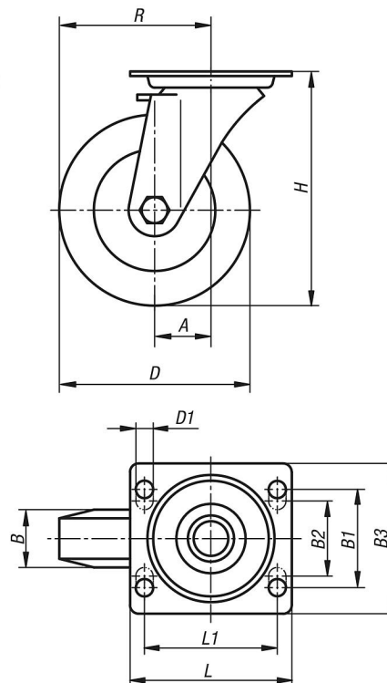
swivel castor
