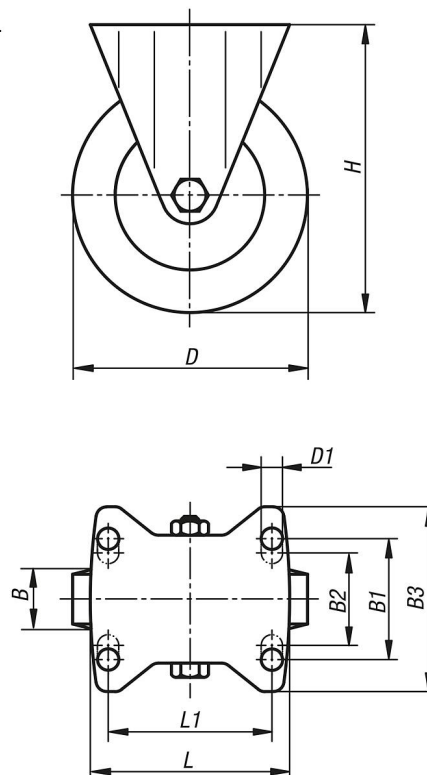
fixed castor
