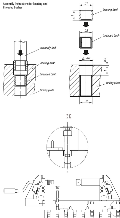
Assembly instructions for locating and threaded bushes
