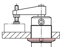
With a slotted round nut from below.
