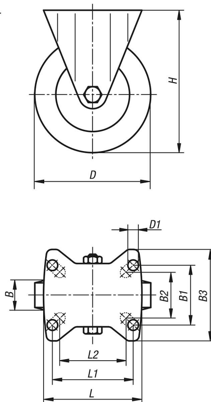
fixed castor
