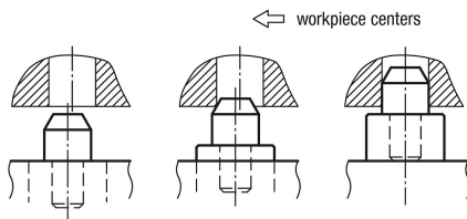
1. roughly position 2. raise pin 3. located
