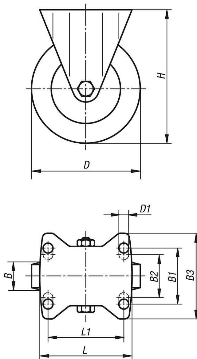
fixed castor
