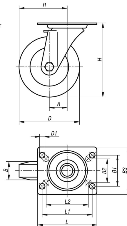
swivel castor
