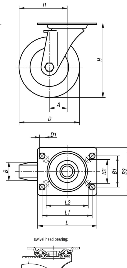
swivel castor
