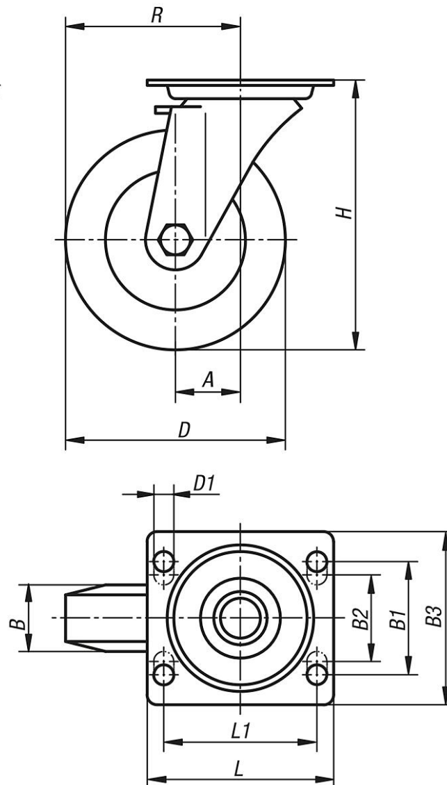
swivel castor
